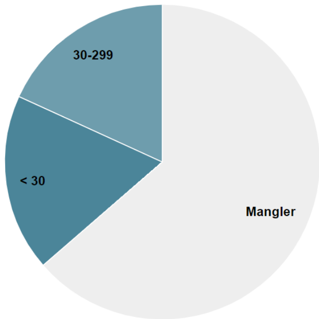
U-alb/kre ratio
